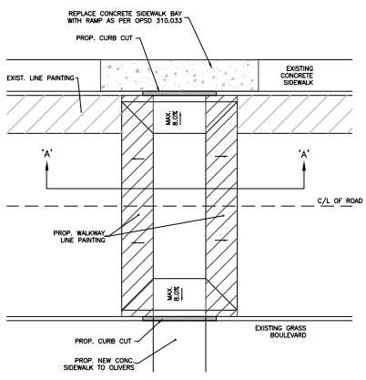
CROSSWALK WITH SPEED BUMP DETAIL SCALE 1:100
